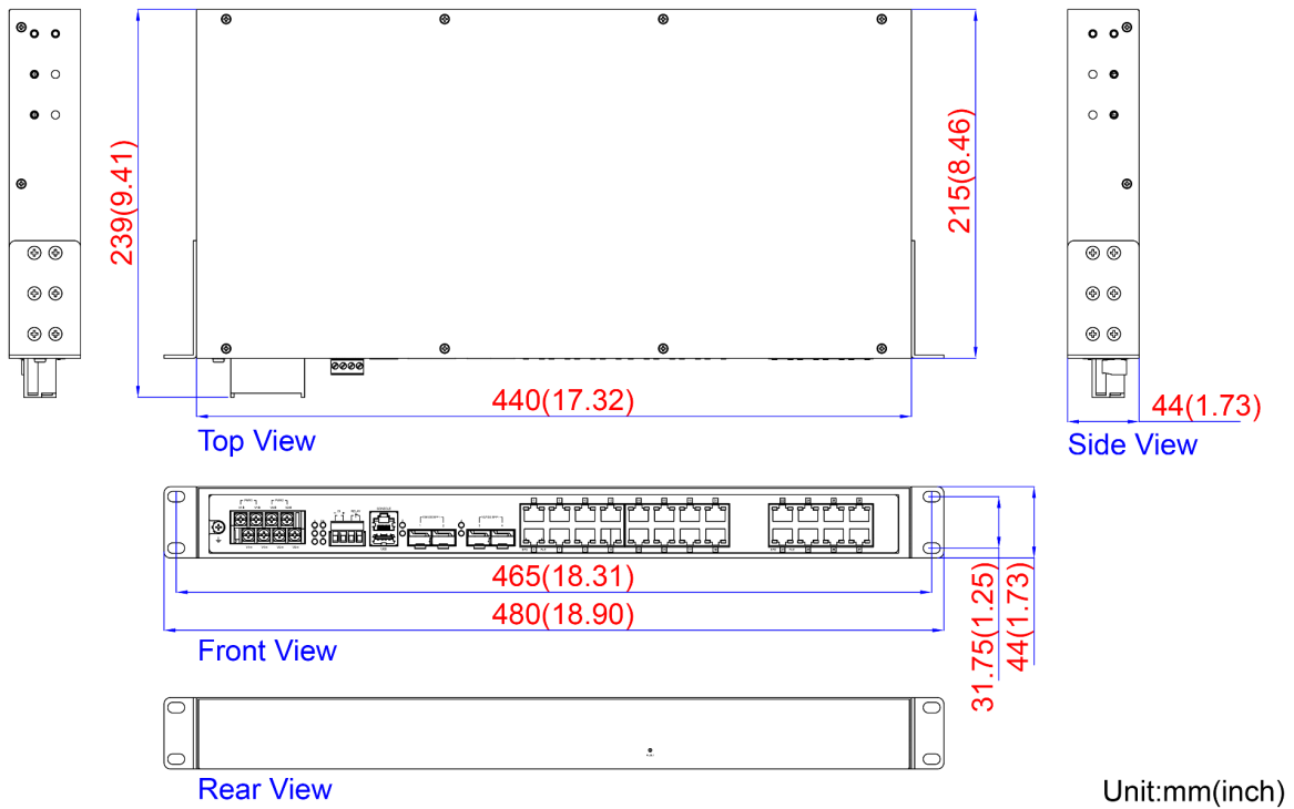
Figure 2.1 - Physical Dimensions
