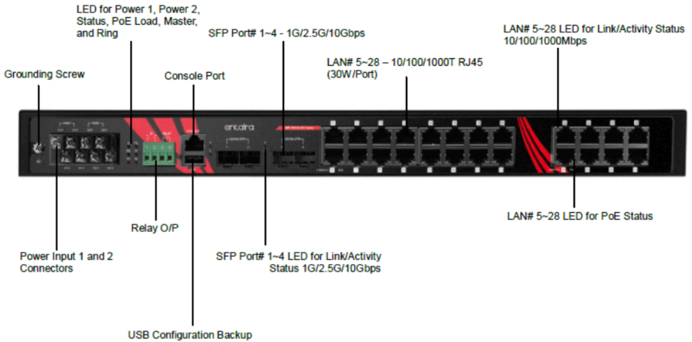
Figure 2.2 - Front View Panel
